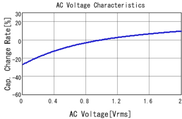
■ GRM21BC71E475KE11 C-AC Voltage capchange, DCOV, 25.0d
