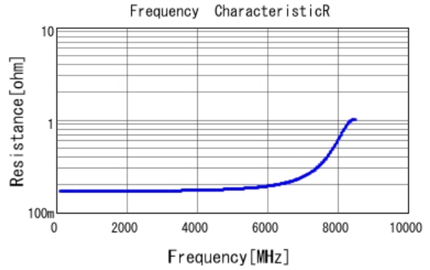
GQM22M5C2H1R1BB01 R DCOV, 25degC
