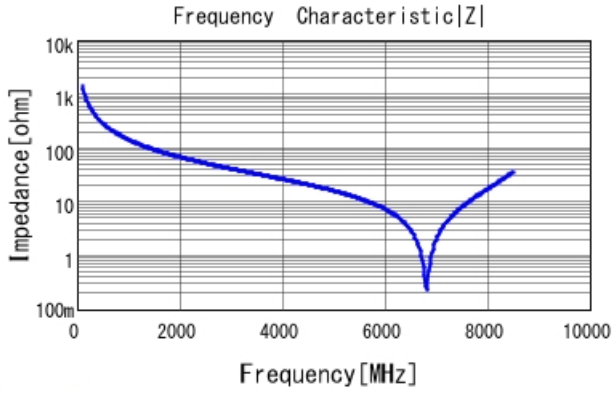
GQM22M5C2H1R1BB01 |Z| DCOV, 25degC
