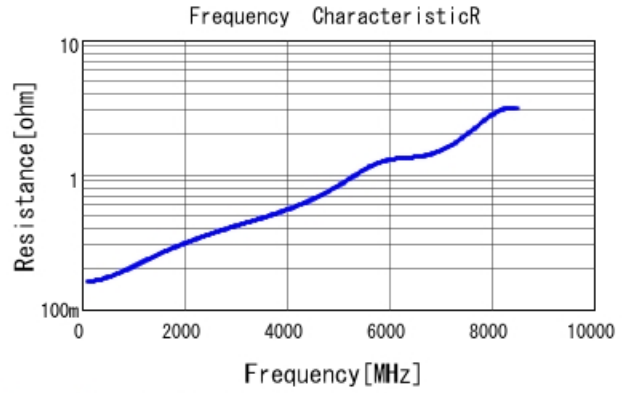
GRM1555C1H9R7CA01 R DCOV, 25degC
