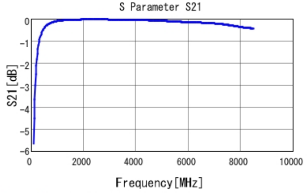
GRM1555C1H9R7CA01 S21 DCOV, 25degC
