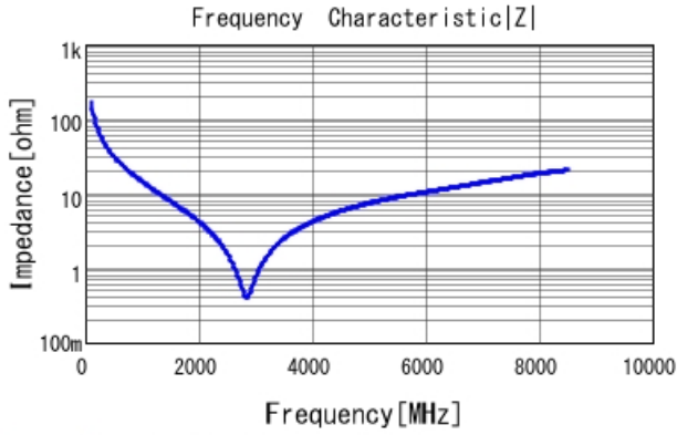
GRM1555C1H9R7CA01 |Z| DCOV, 25degC
