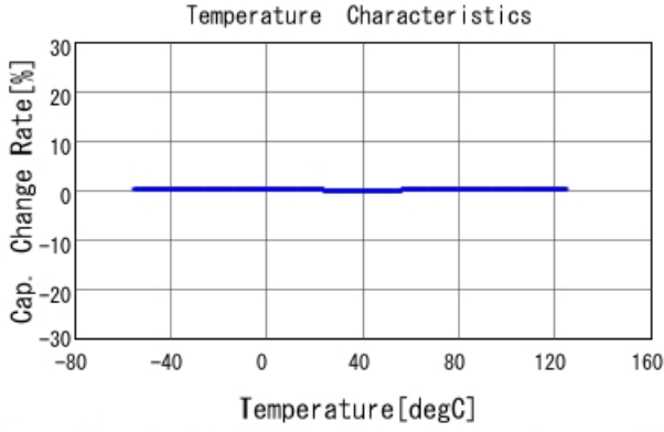
GRM1555C1H9R7CA01 C-Temp. capchange, DCOV, AC1Vrms
