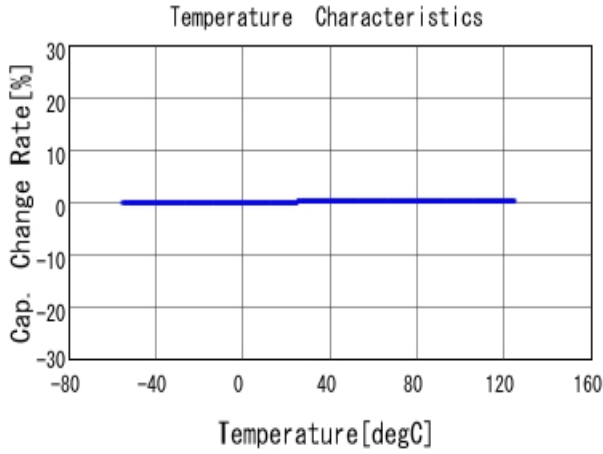
■ GQM2195C2A8R2DB01 C-Temp. capchange, DCOV, AC1Vrms
