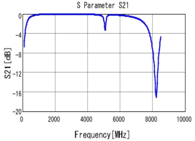
■ GQM2195C2A8R2DB01 S21 DCOV, 25degC
