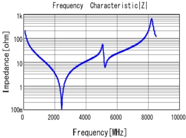
■ GQM2195C2A8R2DB01 |Z| DC0V, 25degC
