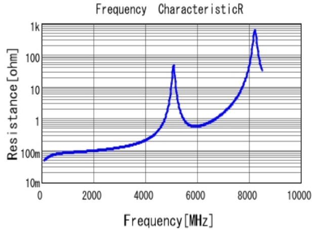
■ GQM2195C2A8R2DB01 R DC0V, 25degC
