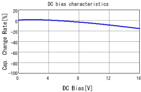
GRM21BR71C474MA01 C-DC bias capchange, 25.0degC, A
