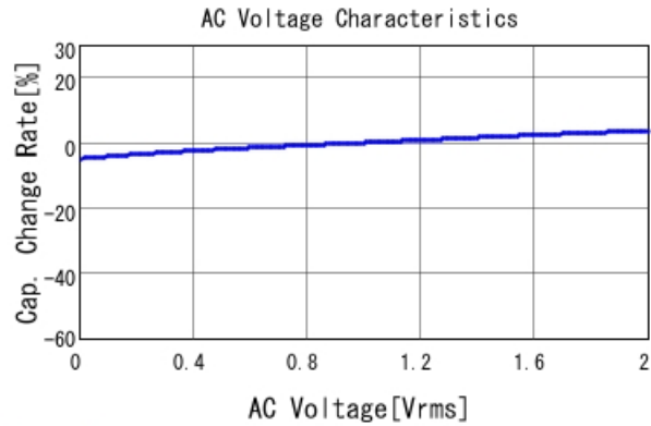
GRM21BR71C474MA01 C-AC Voltage capchange, DCOV, 25
