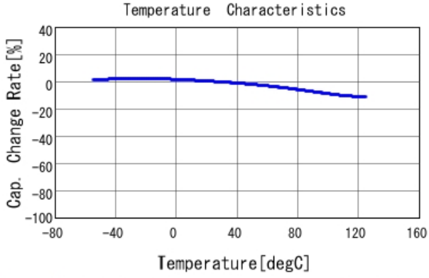
GRM21BR71C474MA01 C-Temp. capchange, DC0.0V, AC1.C
