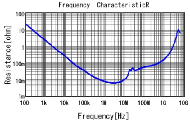
GRM21BR71C474MA01 R DCOV, 25degC
