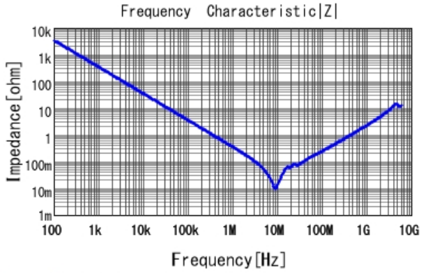
GRM21BR71C474MA01 |Z| DCOV, 25degC
