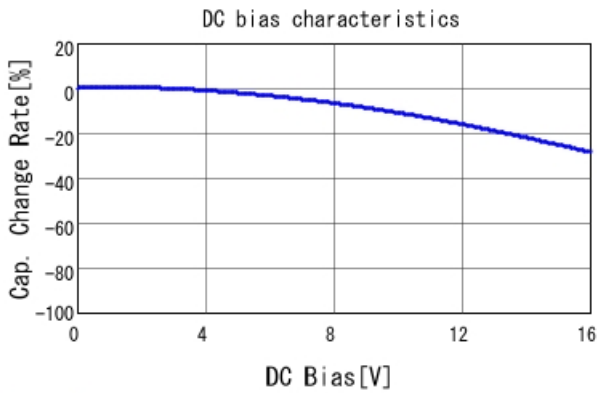
GCJ21BR71C105MA01 C-DC bias capchange, 25.0degC, A
