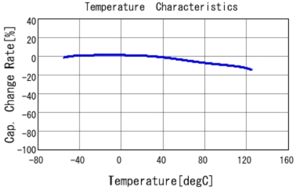
GCJ21BR71C105MA01 C-Temp. capchange, DC0.0V, AC1.C
