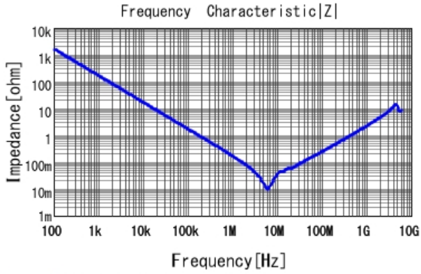
GCJ21BR71C105MA01 |Z| DCOV, 25degC
