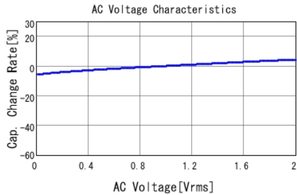
GCJ21BR71C105MA01 C-AC Voltage capchange, DCOV, 25
