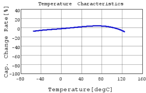
GCJ188R70J225KE01 C-Temp. capchange, DC0.0V,
