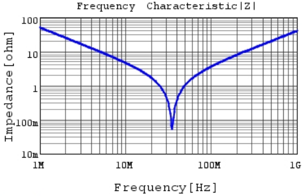
RDE5C1H332J0K1H03B |Z| DC0V, 25degC
