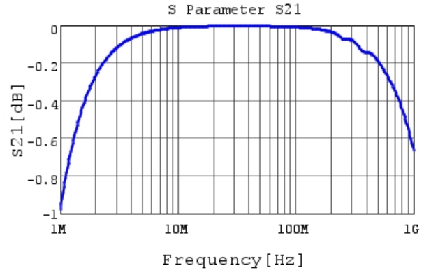
RDE5C1H332J0K1H03B S21 DC0V, 25degC
