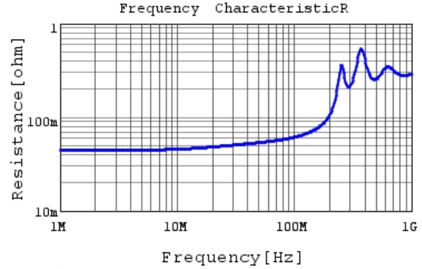
RDE5C1H332J0K1H03B R DC0V, 25degC
