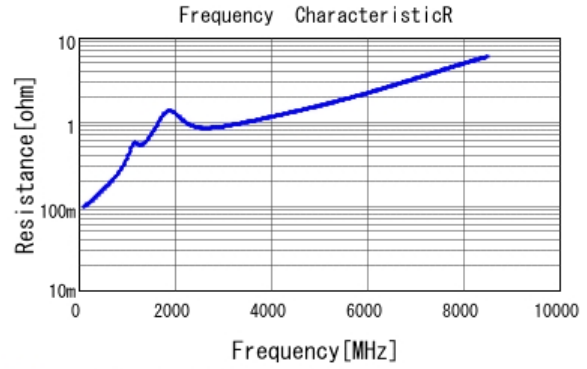
■ GCM1882C1H221JA01 R DCOV, 20degC
