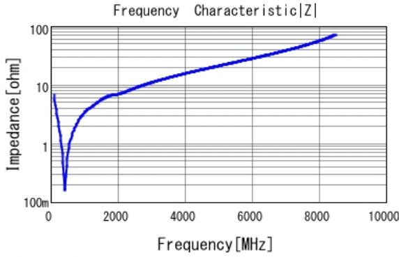
■ GCM1882C1H221JA01 |Z| DCOV, 20degC
