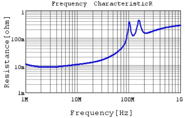
GRM31B5C2E123JWA1 R DC0V, 25degC
