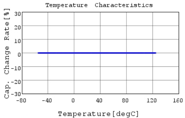
GRM31B5C2E123JWA1 C-Temp. capchange, DC0V, 1
