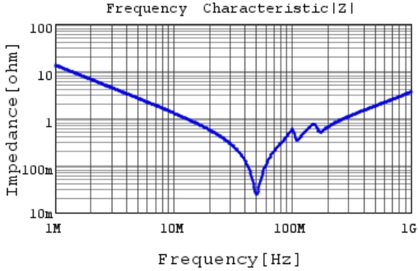
GRM31B5C2E123JWA1 |Z| DC0V, 25degC
