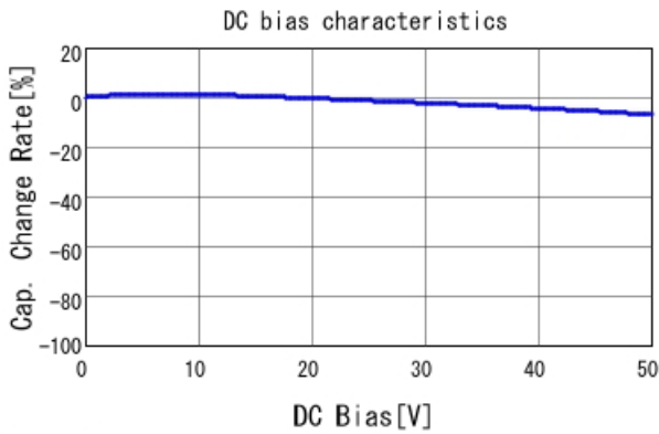
GCE188R71H272KA01 C-DC bias capchange, 25.0degC, A
