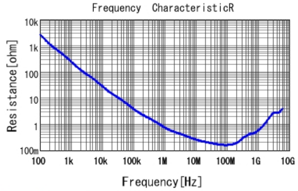
GCE188R71H272KA01 R DCOV, 25degC
