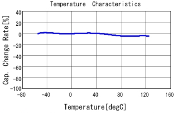
GCE188R71H272KA01 C-Temp. capchange, DC0.0V, AC1.C
