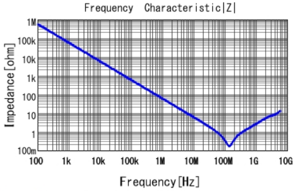
GCE188R71H272KA01 |Z| DCOV, 25degC
