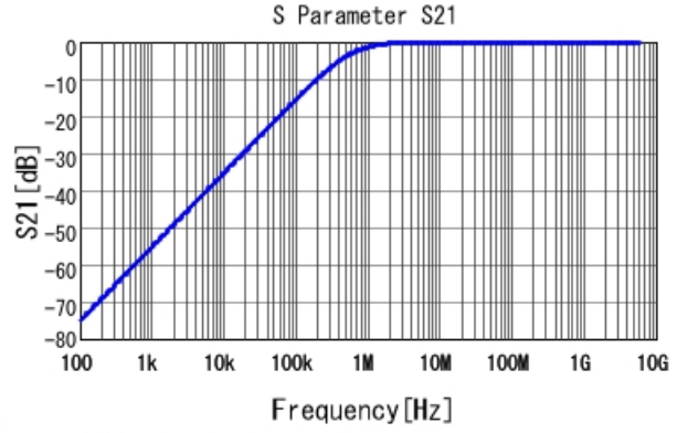
GCE188R71H272KA01 S21 DC0V, 25degC
