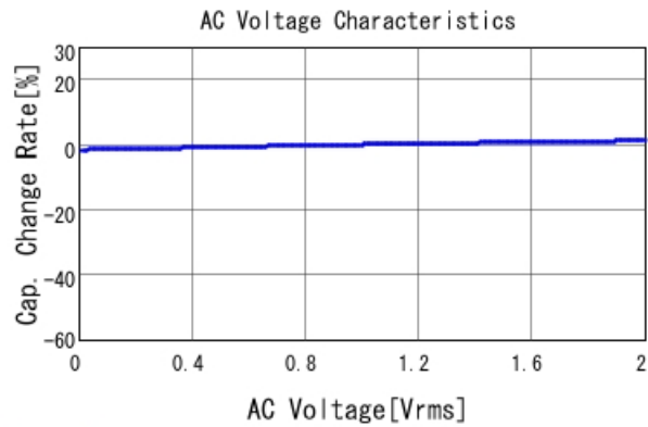
GCE188R71H272KA01 C-AC Voltage capchange, DCOV, 25
