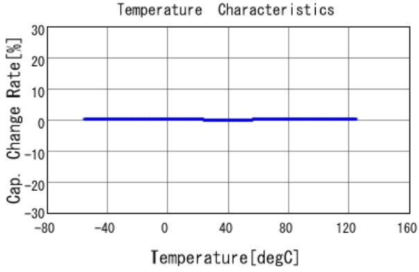
GRM1555C2A6R7DA01 C-Temp. capchange, DCOV, AC1Vrms
