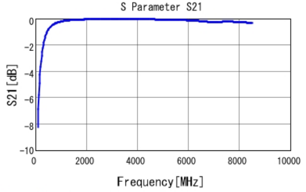
GRM1555C2A6R7DA01 S21 DCOV, 25degC
