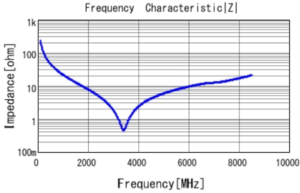
GRM1555C2A6R7DA01 |Z| DCOV, 25degC
