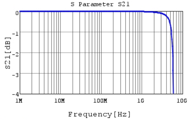
GRM31M7U1H823JA01 S21 DCOV, 25degC
