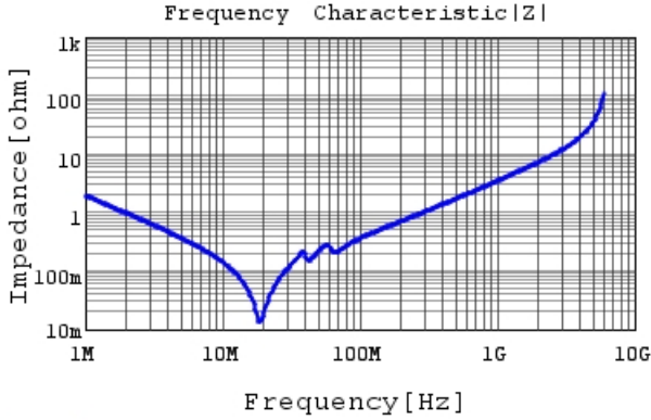
GRM31M7U1H823JA01 |Z| DCOV, 25degC
