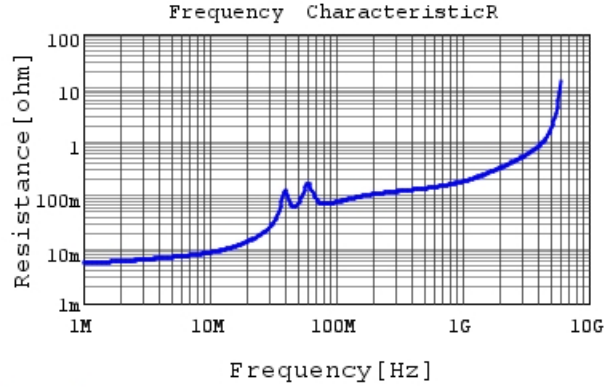
GRM31M7U1H823JA01 R DCOV, 25degC
