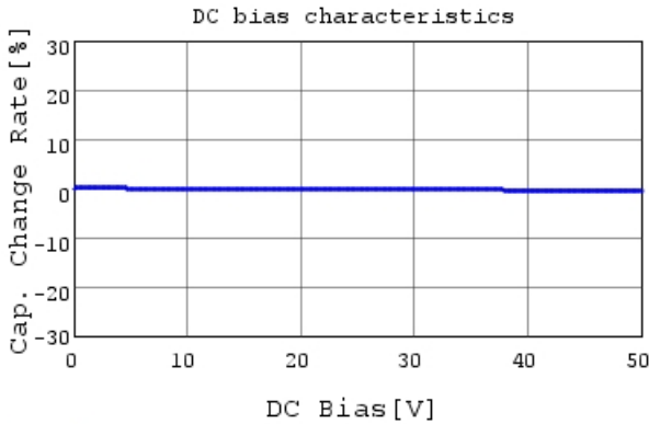
GRM31M7U1H823JA01 C-DC bias capchange, 25.0c
