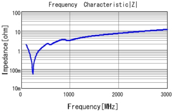
■ GRM21B5C2J681JWA3 |Z| DCOV, 25degC
