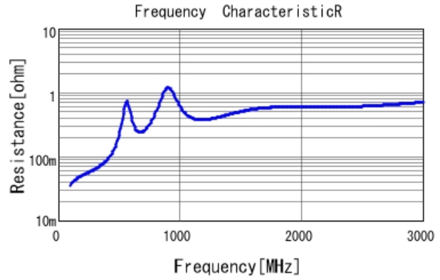
■ GRM21B5C2J681JWA3 R DCOV, 25degC
