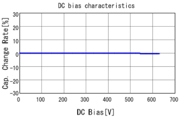
■ GRM21B5C2J681JWA3 C-DC bias capchange, 25.0degC, AC1V
