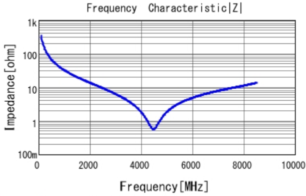
GRM0335C1E4R7CA01 |Z| DCOV, 25degC
