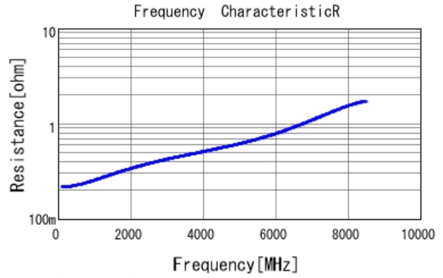
GRM0335C1E4R7CA01 R DCOV, 25degC
