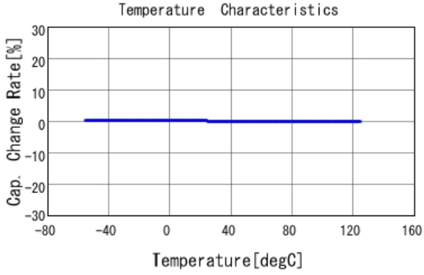
GRM0335C1E4R7CA01 C-Temp. capchange, DCOV, AC1Vrms
