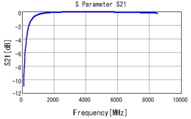
GRM0335C1E4R7CA01 S21 DCOV, 25degC
