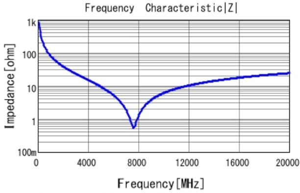
GRM0225C1E1R9WA03 |Z| DCOV, 25degC
