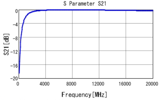
GRM0225C1E1R9WA03 S21 DCOV, 25degC
