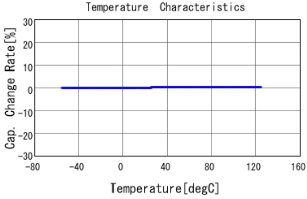
GRM0225C1E1R9WA03 C-Temp. capchange, DCOV, AC1Vrms
