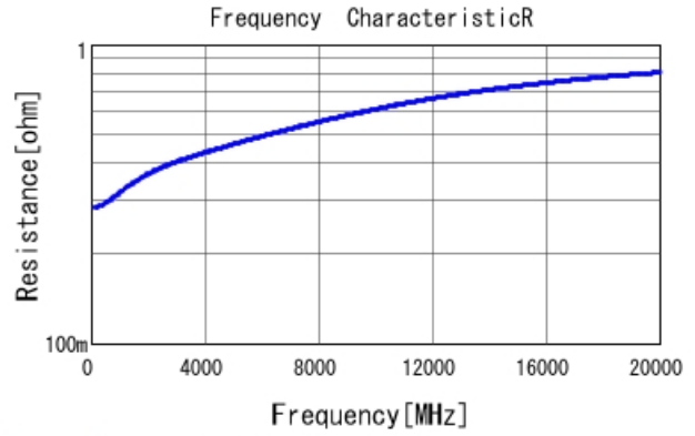
GRM0225C1E1R9WA03 R DCOV, 25degC
