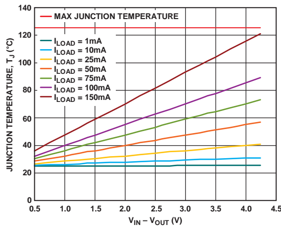
Figure 40. WLCSF, 500 mm 2 of PCB Copper, T_A = 25^\circ\text{C}
