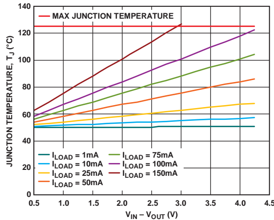
Figure 38. TSOT, 0 mm 2 of PCB Copper, T_A = 50^\circ\text{C}
