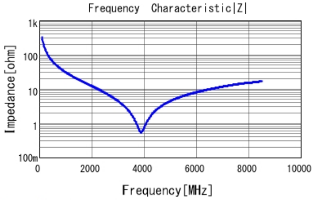
GRM1555C2A4R8WA01 |Z| DCOV, 25degC
