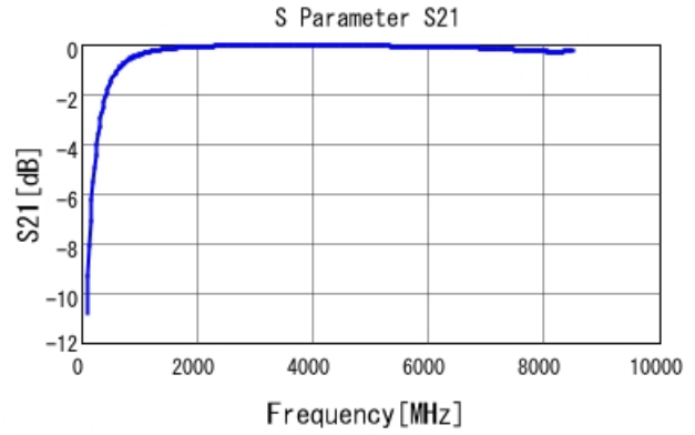
GRM1555C2A4R8WA01 S21 DC0V, 25degC
