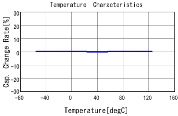
GRM1555C2A4R8WA01 C-Temp. capchange, DC0V, AC1Vrms
