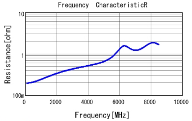
GRM1555C2A7R9WA01 R DCOV, 25degC
