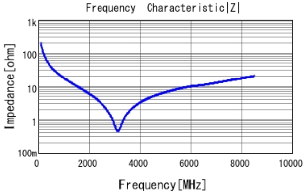
GRM1555C2A7R9WA01 |Z| DCOV, 25degC
