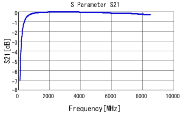
GRM1555C2A7R9WA01 S21 DCOV, 25degC
