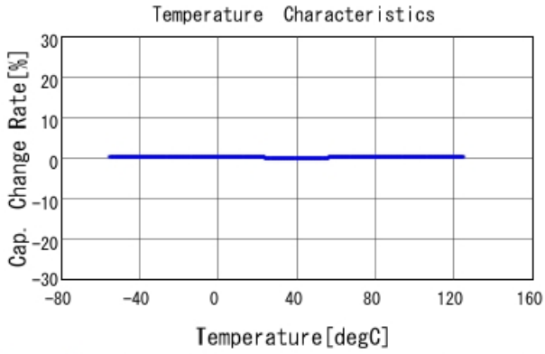
GRM1555C2A7R9WA01 C-Temp. capchange, DCOV, AC1Vrms
