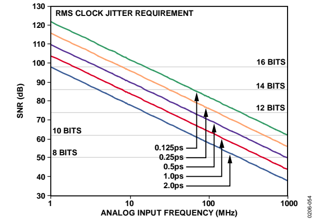
Figure 55. Ideal SNR vs. Input Frequency and Jitter
