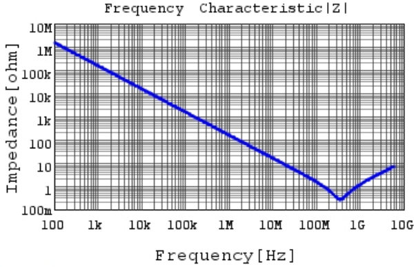
GRM022R71A102MA12 |Z| DCOV, 25degC
