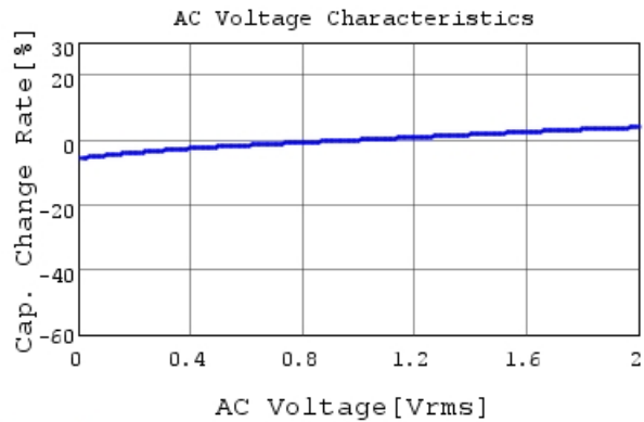
GRM022R71A102MA12 C-AC Voltage capchange, Dc
