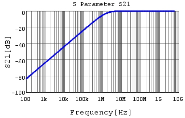
GRM022R71A102MA12 S21 DC0V,25degC
