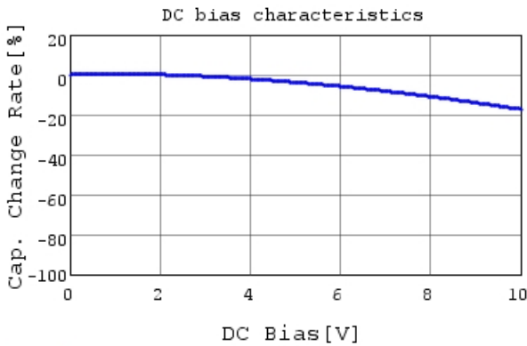
GRM022R71A102MA12 C-DC bias capchange, 25.0c
