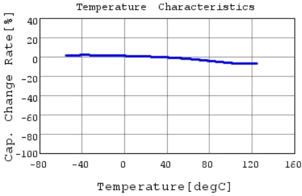
GRM022R71A102MA12 C-Temp. capchange, DC0.0V,
