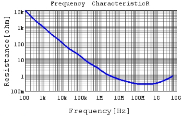
GRM022R71A102MA12 R DCOV, 25degC
