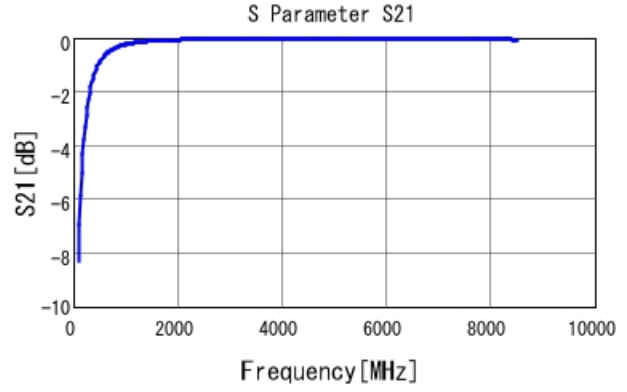
GRM0225C1E6R6DA03 S21 DCOV, 25degC
