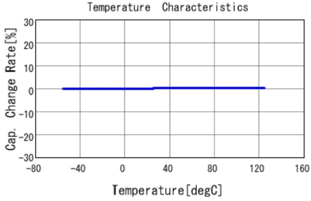
GRM0225C1E6R6DA03 C-Temp. capchange, DCOV, AC1Vrms
