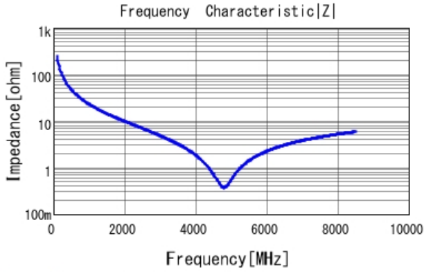
GRM0225C1E6R6DA03 |Z| DCOV, 25degC
