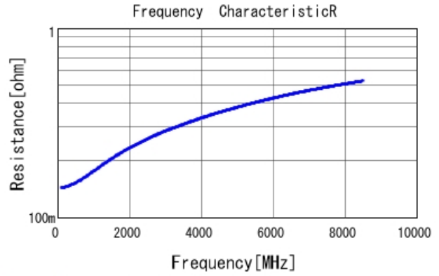
GRM0225C1E6R6DA03 R DCOV, 25degC
