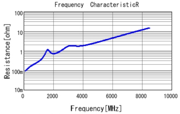
GCM1885C1H820JA16 R DCOV, 25degC
