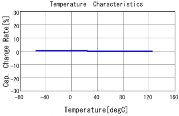
GCM1885C1H820JA16 C-Temp. capchange, DCOV, AC1Vrms
