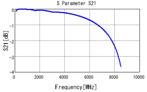
GCM1885C1H820JA16 S21 DCOV, 25degC
