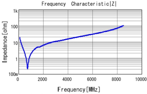
GCM1885C1H820JA16 |Z| DCOV, 25degC
