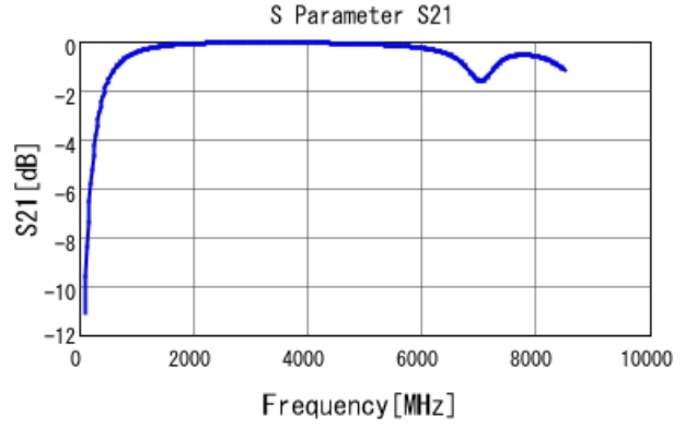
GRM1885C1H4R6BA01 S21 DCOV, 25degC
