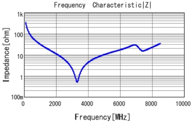
GRM1885C1H4R6BA01 |Z| DCOV, 25degC
