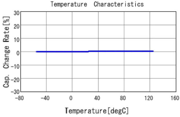
GRM1885C1H4R6BA01 C-Temp. capchange, DCOV, AC1Vrms
