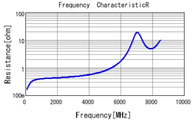
GRM1885C1H4R6BA01 R DCOV, 25degC
