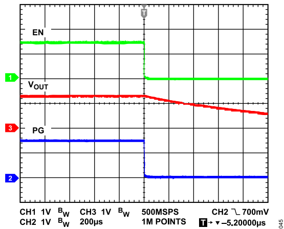
Figure 45. Typical PG Voltage Behavior vs. V_{OUT} , V_{IN} Falling ( V_{OUT} = 1.3\text{ V} )
