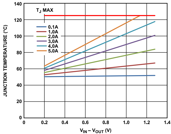
Figure 53. 1000 mm 2 of PCB Copper, T B = 50°C
