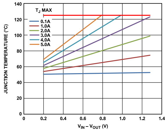
Figure 55. 100 mm 2 of PCB Copper, T B = 50°C
