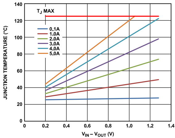
Figure 52. 100 mm 2 of PCB Copper, T B = 25°C
