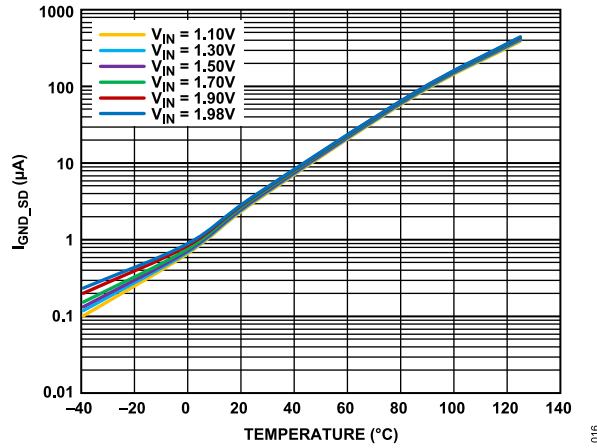
Figure 16. Shutdown Current ( I_{GND\_SD} ) vs. Temperature at Various Input Voltages ( V_{IN} ), V_{OUT} = 0.9\text{ V}
