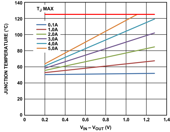
Figure 54. 500 mm 2 of PCB Copper, T B = 50°C
