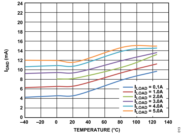
Figure 13. Ground Current ( I_{GND} ) vs. Temperature, V_{OUT} = 0.9 V
