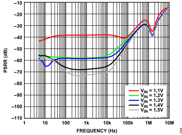
Figure 34. Power Supply Rejection Ratio (PSRR) vs. Frequency at Various Input Voltages ( V_{IN} ), V_{OUT} = 0.9\text{ V} , Load = 5 A
