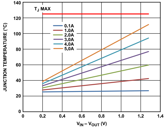
Figure 51. 500 mm 2 of PCB Copper, T B = 25°C
