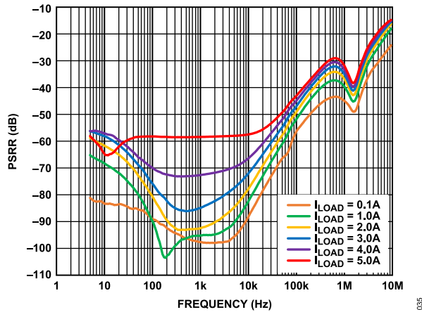
Figure 35. Power Supply Rejection Ratio (PSRR) vs. Frequency at Various Loads ( I_{LOAD} ), V_{OUT} = 0.9\text{ V} , V_{IN} = 1.3\text{ V}
