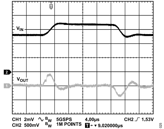
Figure 25. Line Transient Response, Load Current = 5 A, V_{IN} = 1.3 \text{ V} to 1.7 \text{ V} Step, V_{OUT} = 0.9 \text{ V}
