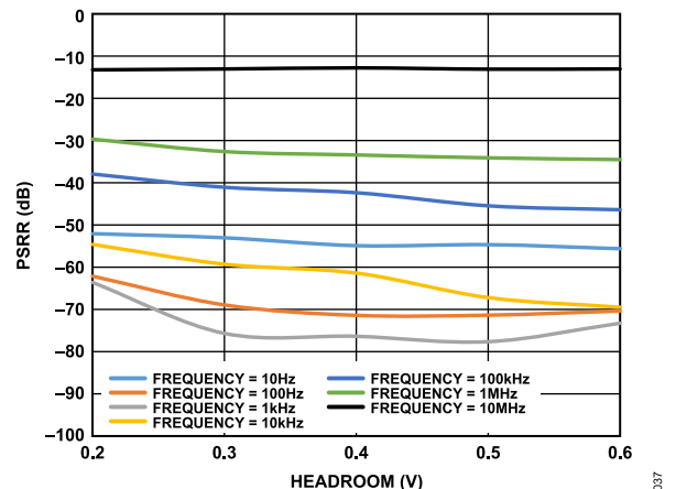
Figure 37. Power Supply Rejection Ratio (PSRR) vs. Headroom Voltage at Various Frequencies, V_{OUT} = 1.3\text{ V} , Load = 5 A
