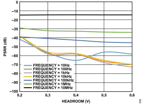
Figure 36. Power Supply Rejection Ratio (PSRR) vs. Headroom Voltage at Various Frequencies, V_{OUT} = 0.9\text{ V} , Load = 5 A
