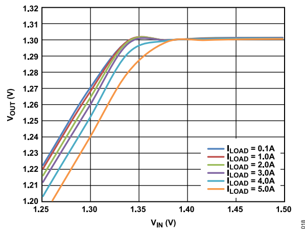
Figure 18. Output Voltage ( V_{OUT} ) vs. Input Voltage ( V_{IN} ) in Dropout, V_{OUT} = 1.3\text{ V}
