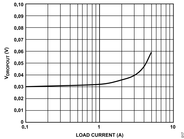
Figure 17. Dropout Voltage ( V_{DROPOUT} ) vs. Load Current ( I_{LOAD} ), V_{OUT} = 1.3\text{ V}
