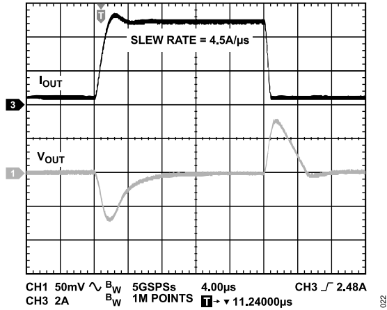
Figure 22. Load Transient Response, C_{OUT} = 22 \mu\text{F} , V_{IN} = 1.4 \text{ V} , V_{OUT} = 0.9 \text{ V}
