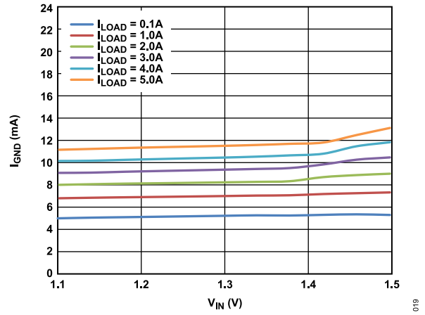
Figure 19. Ground Current ( I_{GND} ) vs. Input Voltage ( V_{IN} ) in Dropout, V_{OUT} = 1.3\text{ V}
