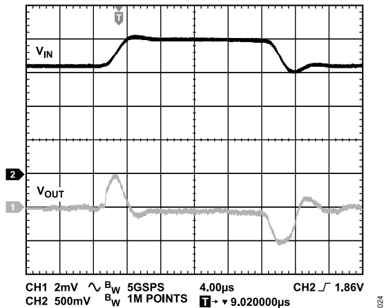
Figure 24. Line Transient Response, Load Current = 5 A, V_{IN} = 1.6 \text{ V} to 1.98 \text{ V} Step, V_{OUT} = 1.3 \text{ V}
