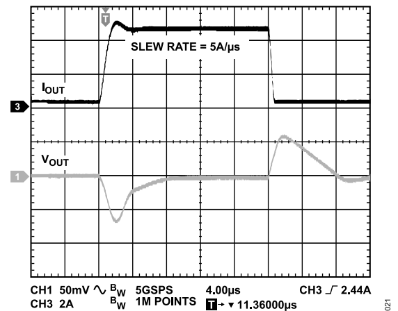
Figure 21. Load Transient Response, C_{OUT} = 47\text{ }\mu\text{F} , V_{IN} = 1.8\text{ V} , V_{OUT} = 1.3\text{ V}
