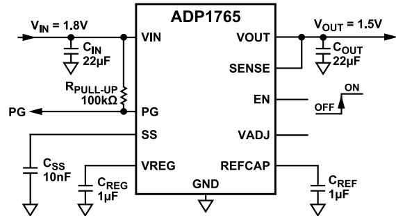
Figure 1. Fixed Output Operation
