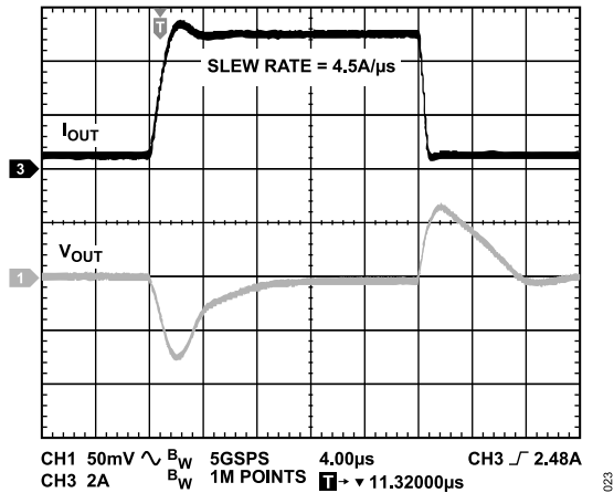
Figure 23. Load Transient Response, C_{OUT} = 47 \mu\text{F} , V_{IN} = 1.4 \text{ V} , V_{OUT} = 0.9 \text{ V}
