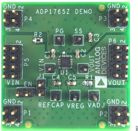
Figure 57. Evaluation Board
