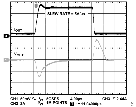
Figure 20. Load Transient Response, C_{OUT} = 22\text{ }\mu\text{F} , V_{IN} = 1.8\text{ V} , V_{OUT} = 1.3\text{ V}
