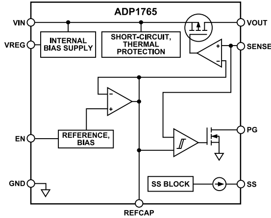
Figure 38. Functional Block Diagram, Fixed Output
