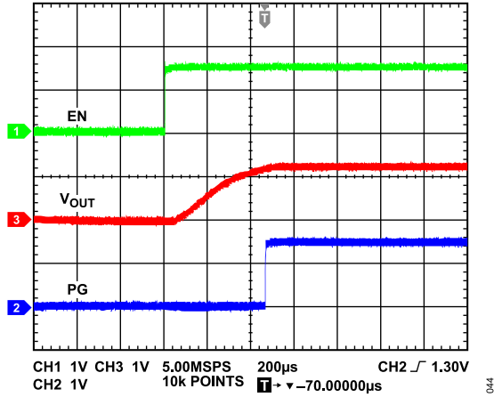
Figure 44. Typical PG Voltage Behavior vs. V_{OUT} , V_{IN} Rising ( V_{OUT} = 1.3\text{ V} )
