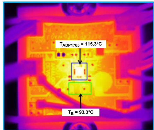
Figure 56. Thermal Image of the ADP1765 Evaluation Board at I LOAD = 5 A, V IN = 1.5 V, V OUT = 1.3 V, T B = 93.3°C
