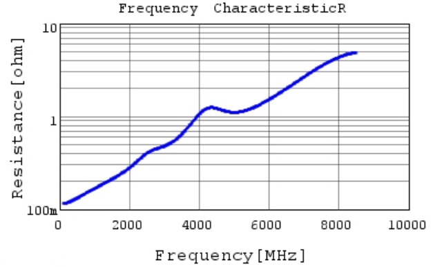
GRM0335C1H820GA01 R DCOV, 25degC
