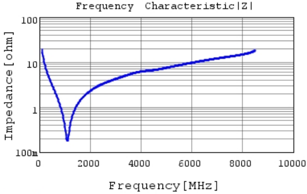
GRM0335C1H820GA01 |Z| DCOV, 25degC
