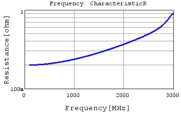
GRM31A5C3A120GW01 R DC0V, 25degC
