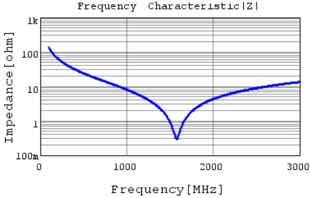
GRM31A5C3A120GW01 |Z| DC0V, 25degC
