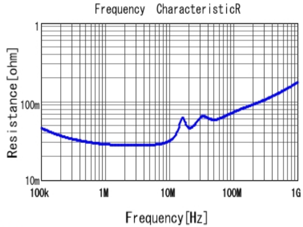
■ RCER72A474K2DBH03A R DC0V, 25degC
