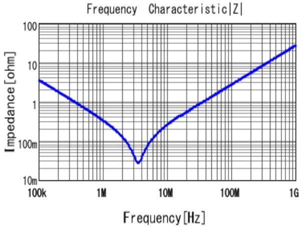
■ RCER72A474K2DBH03A |Z| DC0V, 25degC
