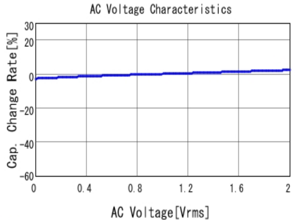
■ RCER72A474K2DBH03A C-AC Voltage capchange, DC0V, 25.0
