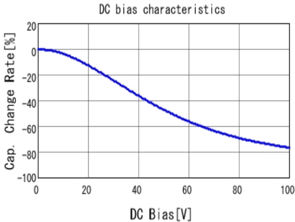
■ RCER72A474K2DBH03A C-DC bias capchange, 25.0degC, AC1
