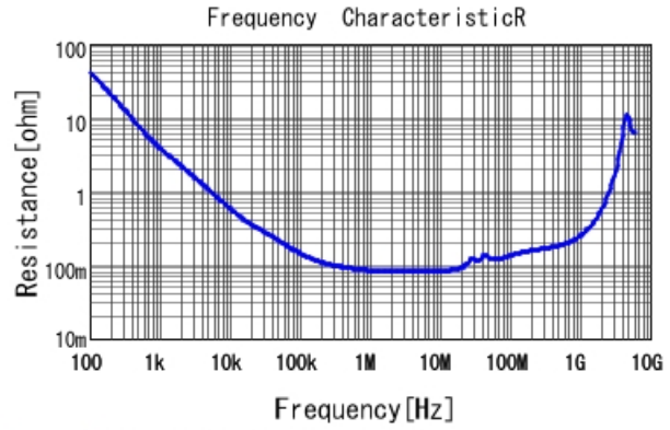
GCJ21BL8YA224KA01 R DCOV, 25degC
