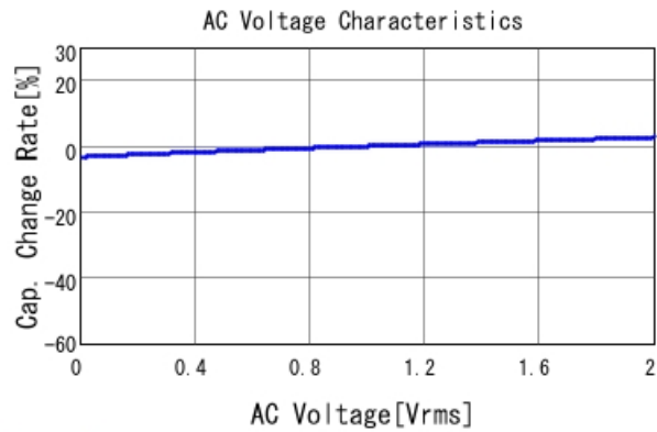
GCJ21BL8YA224KA01 C-AC Voltage capchange, DCOV, 25
