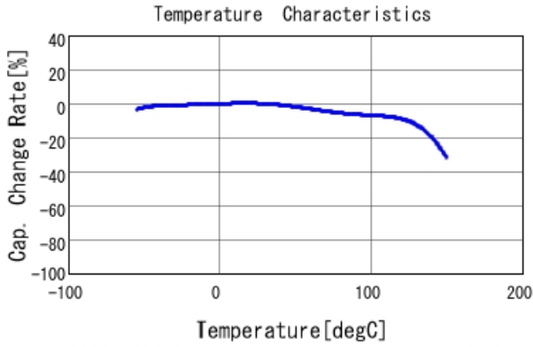
GCJ21BL8YA224KA01 C-Temp. capchange, DC0.0V, AC1.C
