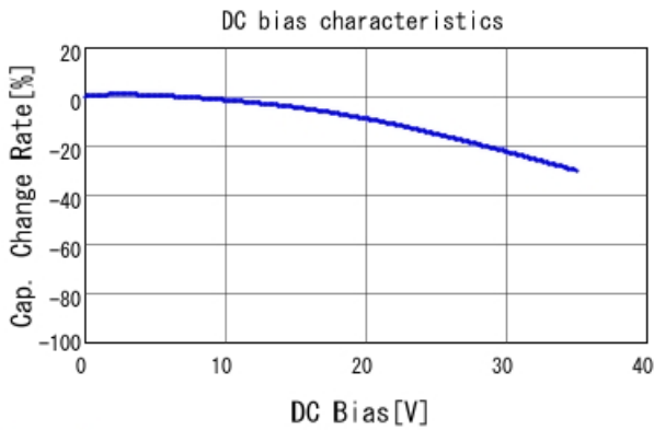
GCJ21BL8YA224KA01 C-DC bias capchange, 25.0degC, A
