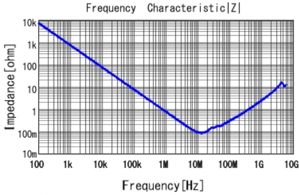
GCJ21BL8YA224KA01 |Z| DCOV, 25degC
