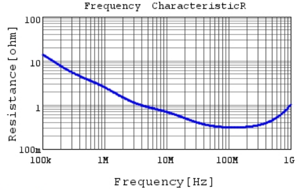
RDER72A102K0S1H03A R DC0V, 25degC
