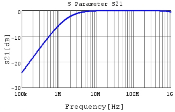
RDER72A102K0S1H03A S21 DC0V, 25degC
