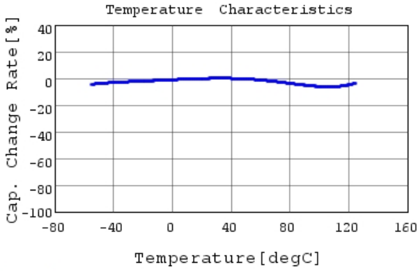
RDER72A102K0S1H03A C-Temp. capchange, DC0.0V
