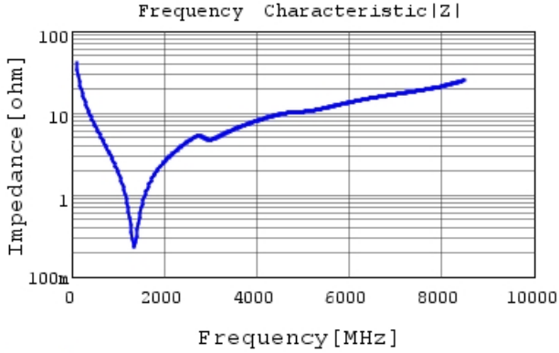
GCM1555C1H390JA16 |Z| DC0V, 25degC
