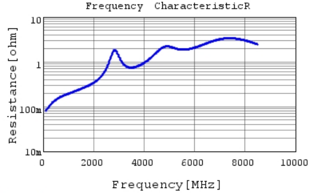
GCM1555C1H390JA16 R DC0V, 25degC
