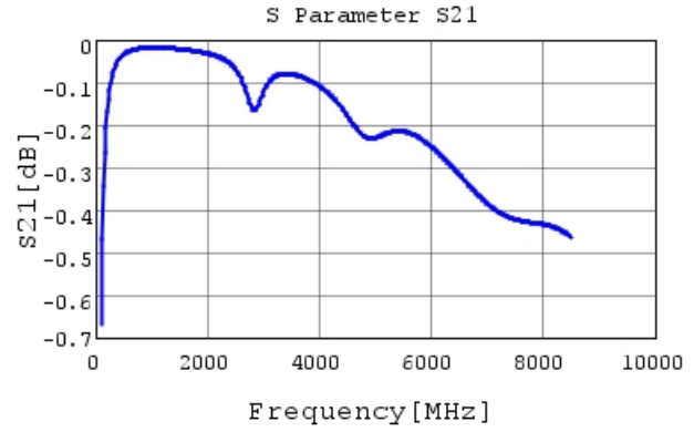
GCM1555C1H390JA16 S21 DCOV, 25degC
