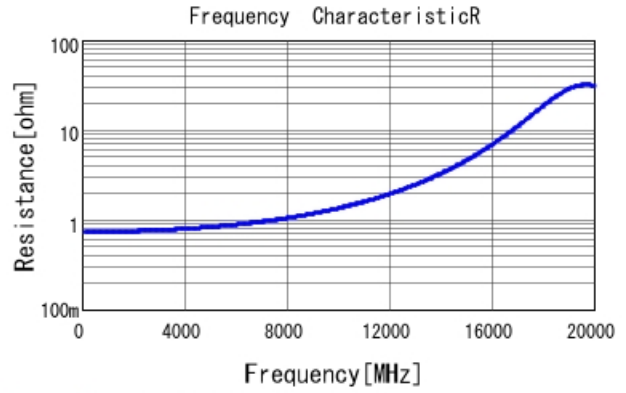
GRM1555C1H1R0WA01 R DCOV, 25degC
