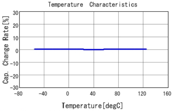
GRM1555C1H1R0WA01 C-Temp. capchange, DCOV, AC1Vrms
