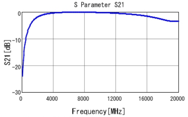
GRM1555C1H1R0WA01 S21 DCOV, 25degC
