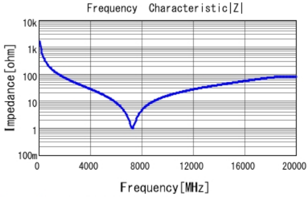
GRM1555C1H1R0WA01 |Z| DCOV, 25degC
