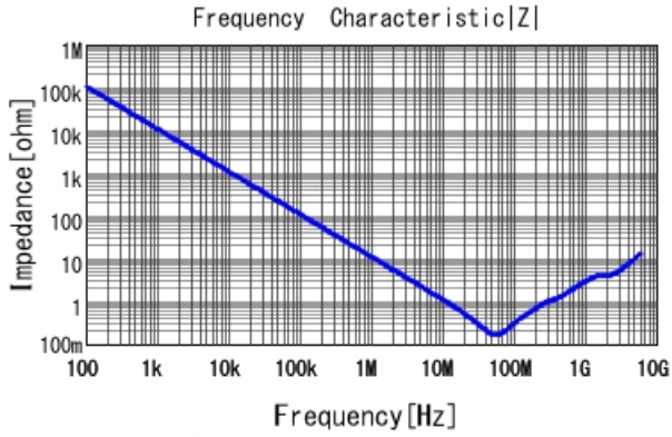
GCJ216R71H153KA01 |Z| DCOV, 25degC
