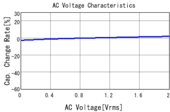
GCJ216R71H153KA01 C-AC Voltage capchange, DCOV, 25
