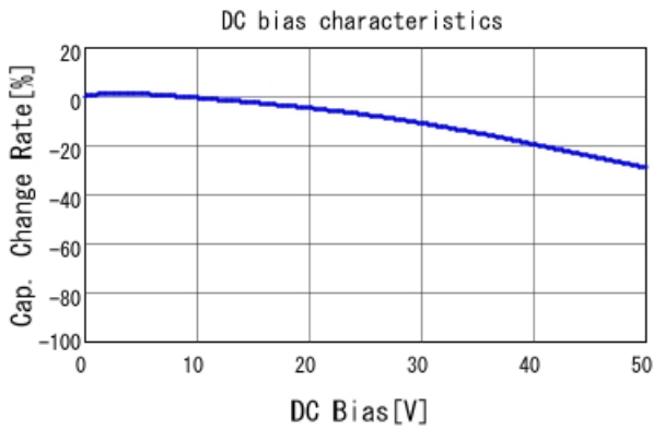
GCJ216R71H153KA01 C-DC bias capchange, 25.0degC, A
