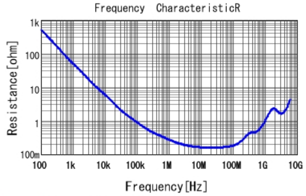
GCJ216R71H153KA01 R DCOV, 25degC
