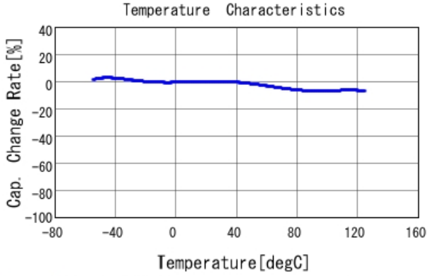
GCJ216R71H153KA01 C-Temp. capchange, DC0.0V, AC1.C
