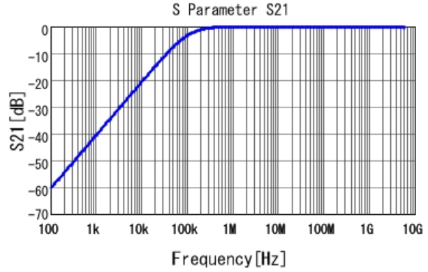
GCJ216R71H153KA01 S21 DC0V, 25degC
