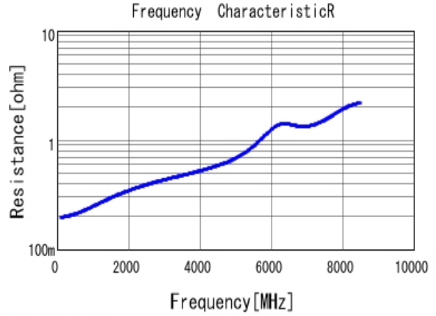
■ GRM1555C2A8R1CA01 R DCOV, 25degC
