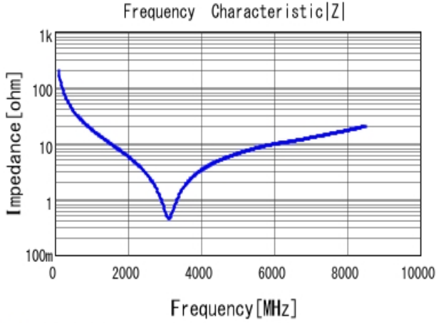
■ GRM1555C2A8R1CA01 |Z| DCOV, 25degC
