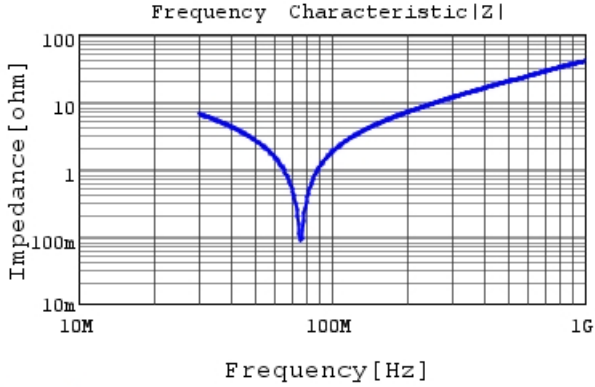
RDE5C2A681J0M1H03A |Z| DCOV, 25degC
