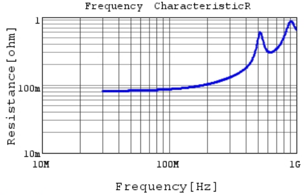
RDE5C2A681J0M1H03A R DCOV, 25degC
