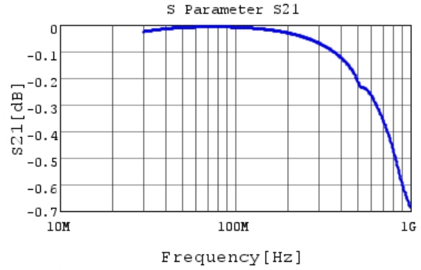
RDE5C2A681J0M1H03A S21 DC0V, 25degC
