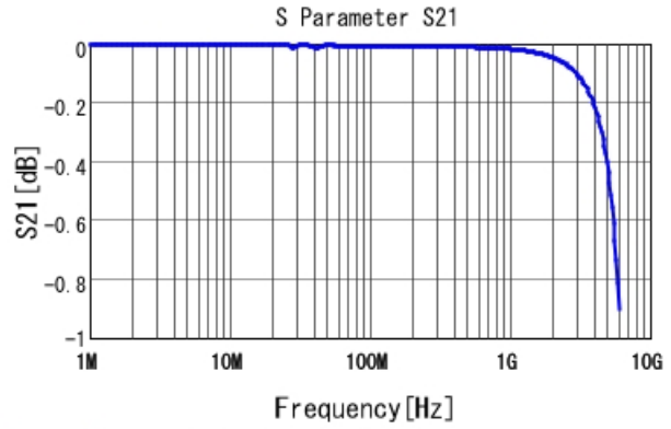
GRM31C5C1C124JA01 S21 DCOV, 25degC
