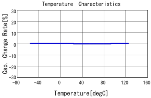
GRM31C5C1C124JA01 C-Temp. capchange, DCOV, AC1Vrms
