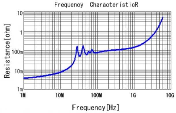
GRM31C5C1C124JA01 R DCOV, 25degC
