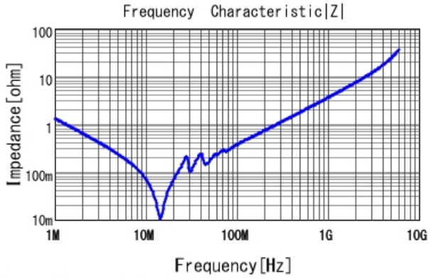
GRM31C5C1C124JA01 |Z| DCOV, 25degC
