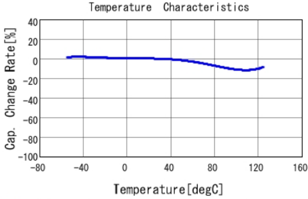
■ GA355QR7GF222KW01 C-Temp. capchange, DCOV, AC1Vrms
