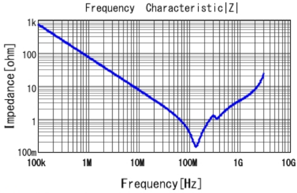
■ GA355QR7GF222KW01 |Z| DC0V, 25degC
