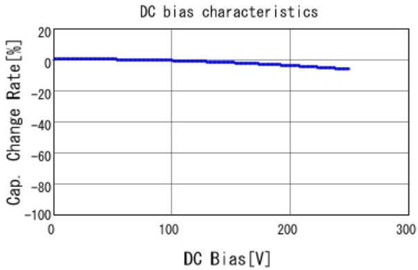
■ GA355QR7GF222KW01 C-DC bias capchange, 25.0degC, AC1V
