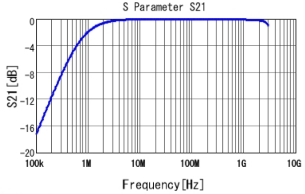
■ GA355QR7GF222KW01 S21 DCOV, 25degC
