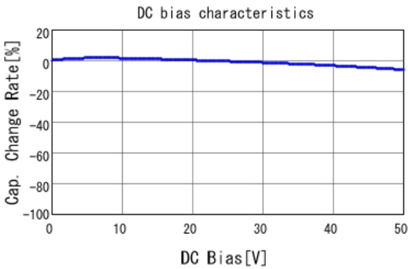
GRM319R71H153KA01 C-DC bias capchange, 25.0degC, A
