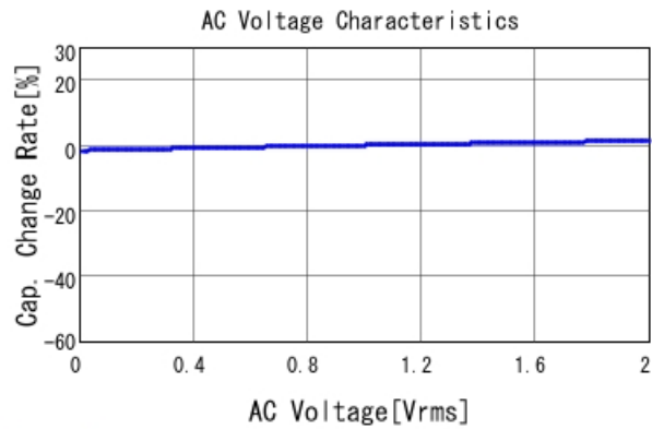
GRM319R71H153KA01 C-AC Voltage capchange, DCOV, 25
