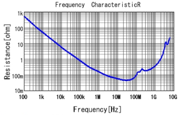
GRM319R71H153KA01 R DCOV, 25degC
