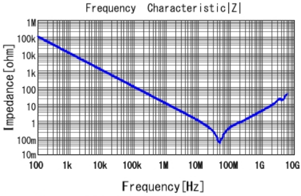
GRM319R71H153KA01 |Z| DCOV, 25degC
