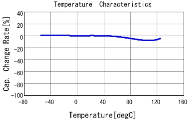
GRM319R71H153KA01 C-Temp. capchange, DC0.0V, AC1.C
