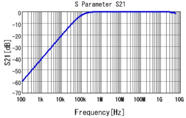
GRM319R71H153KA01 S21 DC0V, 25degC
