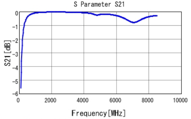
GRM1885C1H9R8BA01 S21 DCOV, 25degC
