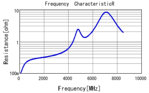
GRM1885C1H9R8BA01 R DCOV, 25degC
