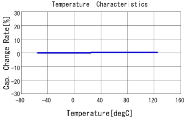
GRM1885C1H9R8BA01 C-Temp. capchange, DCOV, AC1Vrms
