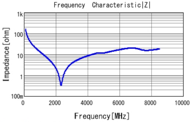
GRM1885C1H9R8BA01 |Z| DCOV, 25degC
