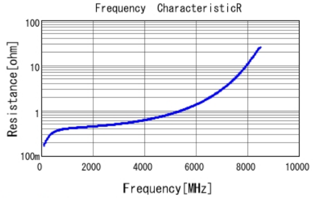
GRM1885C2A2R6WA01 R DCOV, 25degC
