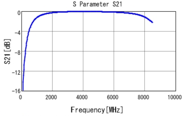
GRM1885C2A2R6WA01 S21 DCOV, 25degC
