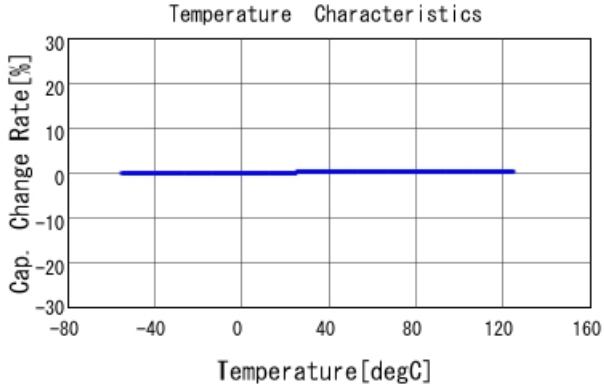
GRM1885C2A2R6WA01 C-Temp. capchange, DCOV, AC1Vrms
