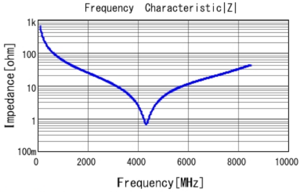
GRM1885C2A2R6WA01 |Z| DCOV, 25degC
