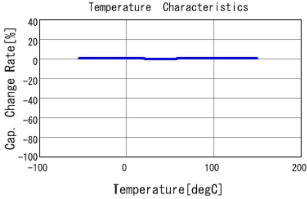
GCM1555G1H821JA16 C-Temp. capchange, DCOV, AC1Vrms
