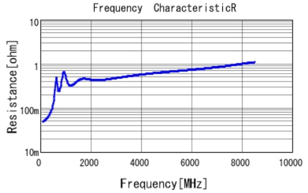
GCM1555G1H821JA16 R DCOV, 25degC
