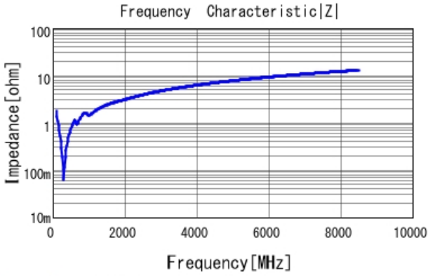
GCM1555G1H821JA16 |Z| DCOV, 25degC
