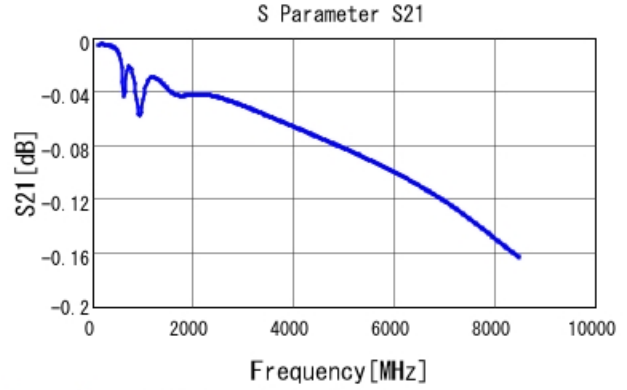
GCM1555G1H821JA16 S21 DCOV, 25degC
