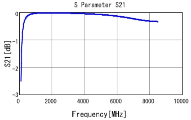
■ GRM0335C1H180GA01 S21 DCOV, 25degC
