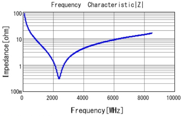
■ GRM0335C1H180GA01 |Z| DCOV, 25degC
