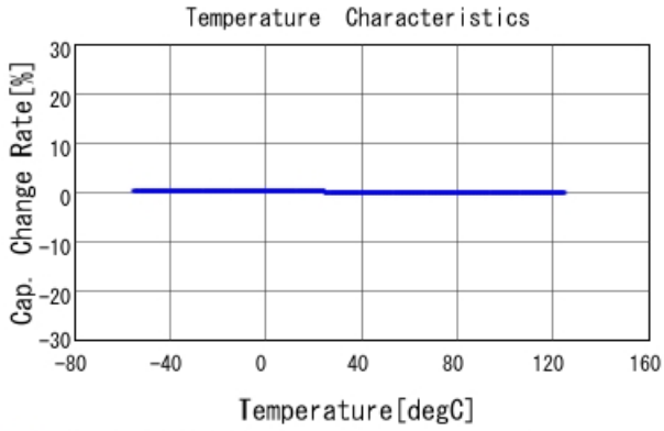
■ GRM0335C1H180GA01 C-Temp. capchange, DCOV, AC1Vrms
