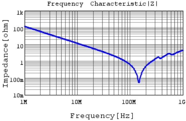
GRM31A5C2J152FWA1 |Z| DCOV,25degC
