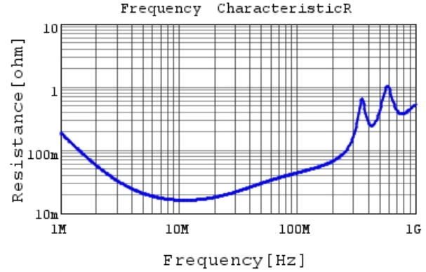
GRM31A5C2J152FWA1 R DCOV,25degC
