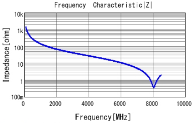
GJM1555C1H1R1WB01 |Z| DCOV, 25degC
