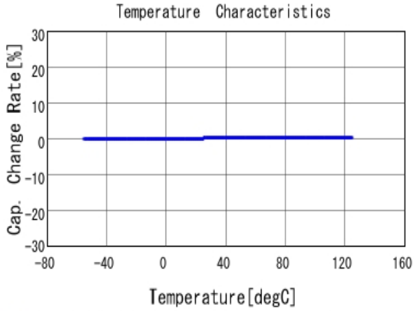
■ GQM2195C2A150JB01 C-Temp. capchange, DCOV, AC1Vrms
