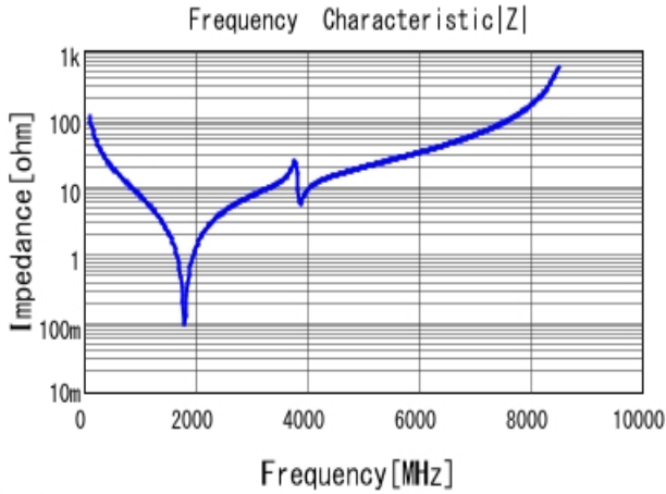
■ GQM2195C2A150JB01 |Z| DC0V, 25degC
