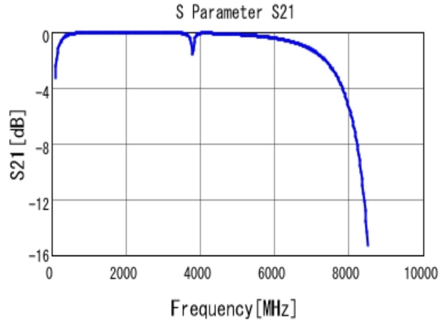
■ GQM2195C2A150JB01 S21 DCOV, 25degC
