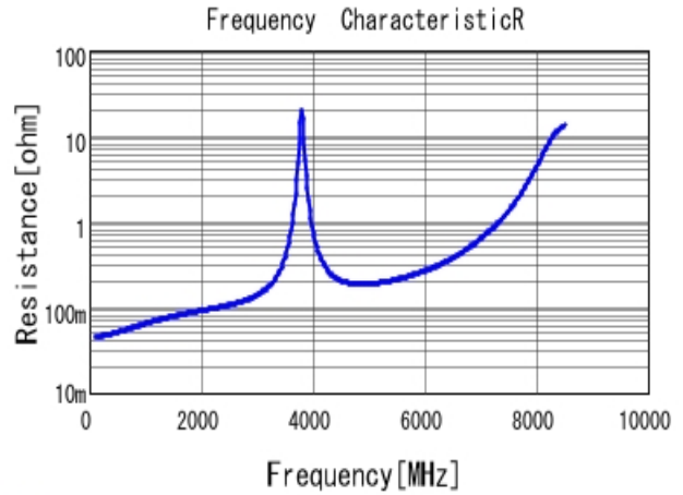
■ GQM2195C2A150JB01 R DC0V, 25degC
