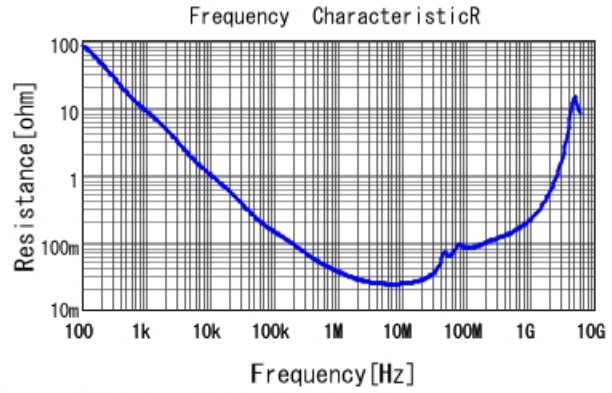
GCJ21BR72A823KA01 R DCOV, 25degC
