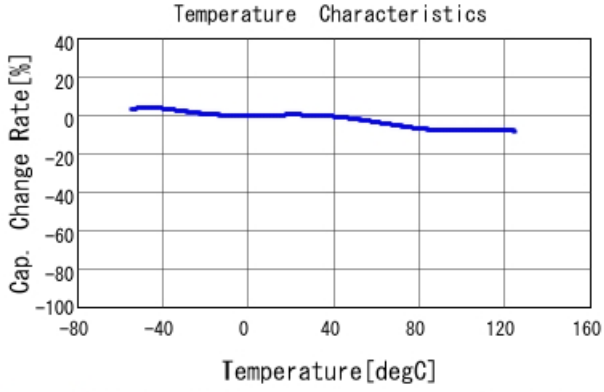
GCJ21BR72A823KA01 C-Temp. capchange, DC0.0V, AC1.C
