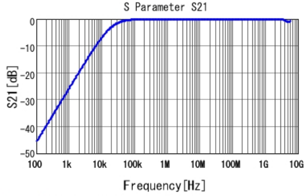
GCJ21BR72A823KA01 S21 DC0V, 25degC
