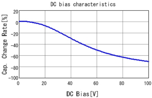
GCJ21BR72A823KA01 C-DC bias capchange, 25.0degC, A
