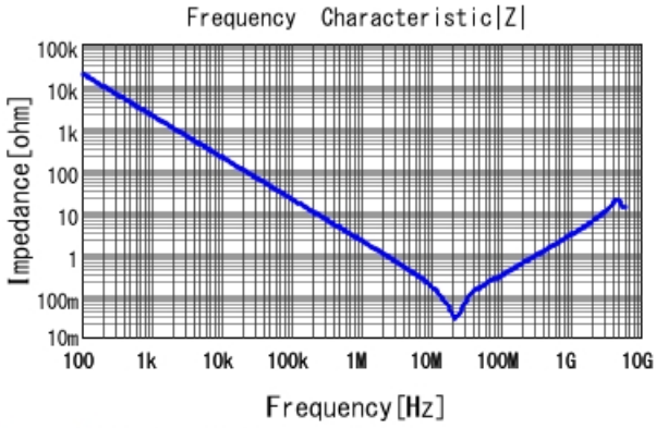
GCJ21BR72A823KA01 |Z| DCOV, 25degC
