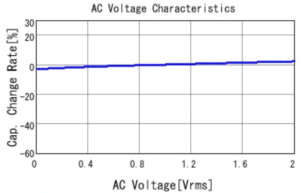
GCJ21BR72A823KA01 C-AC Voltage capchange, DCOV, 25
