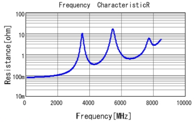
GQM1555C2D330GB01 R DCOV, 25degC
