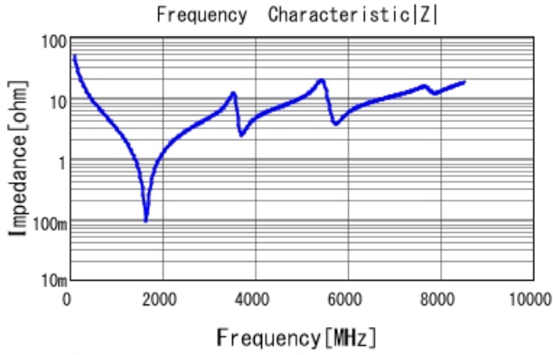
GQM1555C2D330GB01 |Z| DCOV, 25degC
