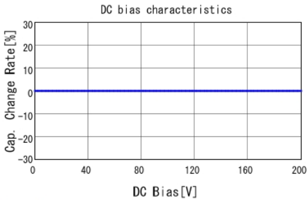
GQM1555C2D330GB01 C-DC bias capchange, 25.0degC, A
