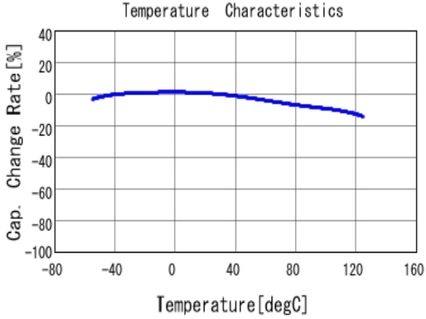
■ GCE188R71E333KA01 C-Temp. capchange, DCO. 0V, AC1.0V rm
