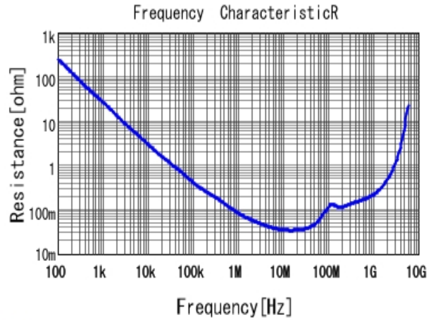
■ GCE188R71E333KA01 R DCOV, 25degC
