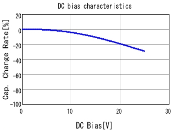
■ GCE188R71E333KA01 C-DC bias capchange, 25.0degC, AC1.
