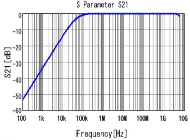
■ GCE188R71E333KA01 S21 DCOV, 25degC
