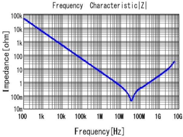
■ GCE188R71E333KA01 |Z| DCOV, 25degC
