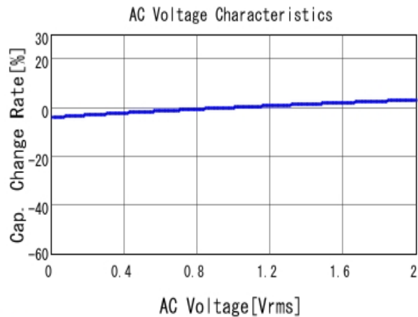
■ GCE188R71E333KA01 C-AC Voltage capchange, DCOV, 25.0d
