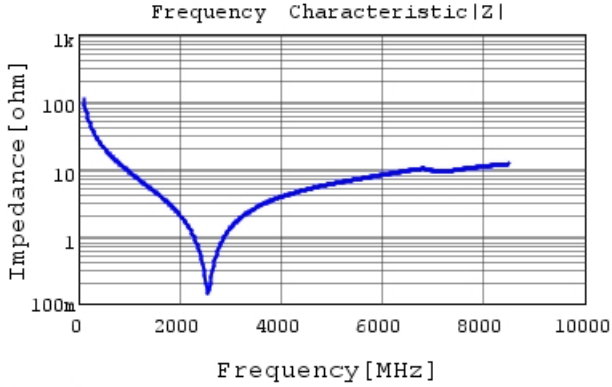
GJM0335C1E150JB01 |Z| DC0V, 25degC
