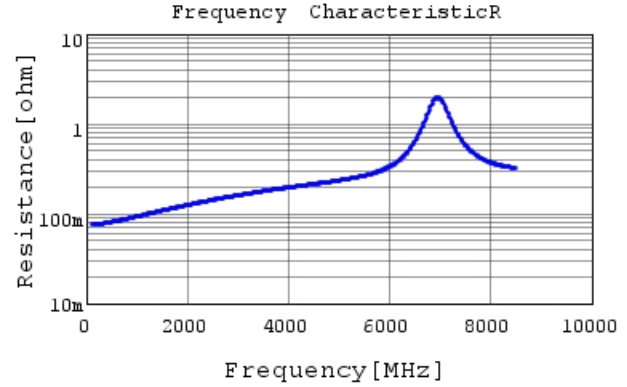
GJM0335C1E150JB01 R DC0V, 25degC
