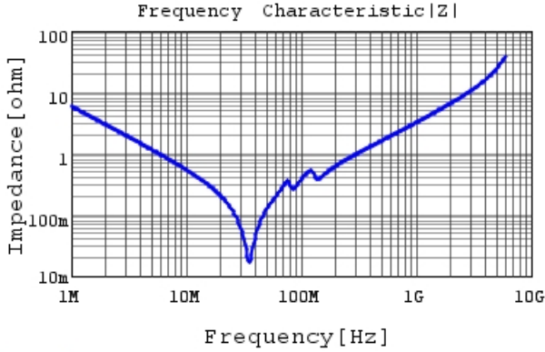
GRM3195C1H273JA01 |Z| DCOV, 25degC
