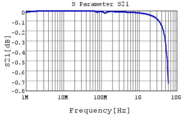
GRM3195C1H273JA01 S21 DCOV, 25degC
