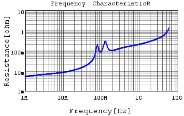
GRM3195C1H273JA01 R DCOV, 25degC
